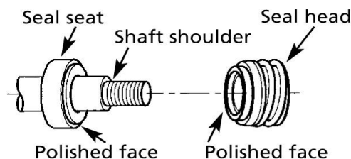
Figure 1 – Mechanical Seal Replacement
