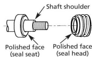
Figure 1 – Seal Replacement
