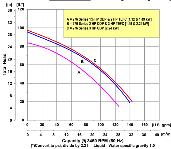
Performance of Stainless Steel Self-Priming Centrifugal Pumps
